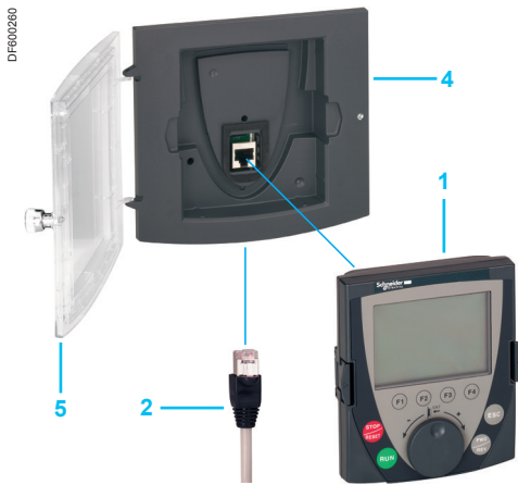
Using the graphic terminal on enclosure door: 1 + 2 + 4 (+ 5, if IP 65)
